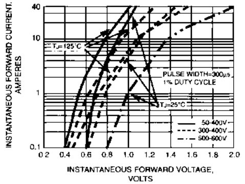
FIG. 4 - TYPICAL INSTANTANEOUS FORWARD CHARACTERISTICS PER LEG
