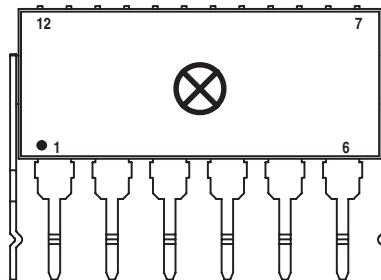
WINGBACK PACKAGE
