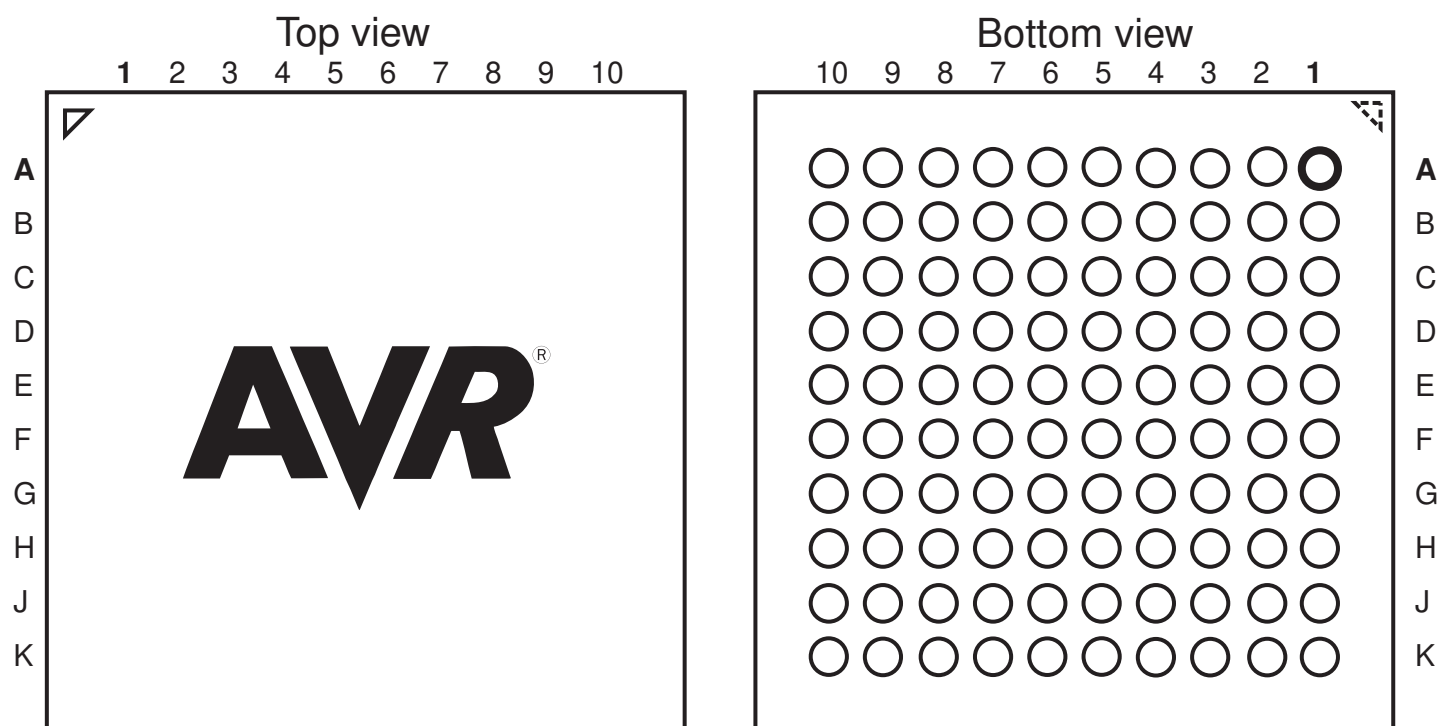
Figure 2-2. CBGA-pinout
