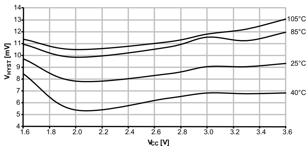
Figure 37-301. Analog comparator hysteresis vs. V_{CC}
