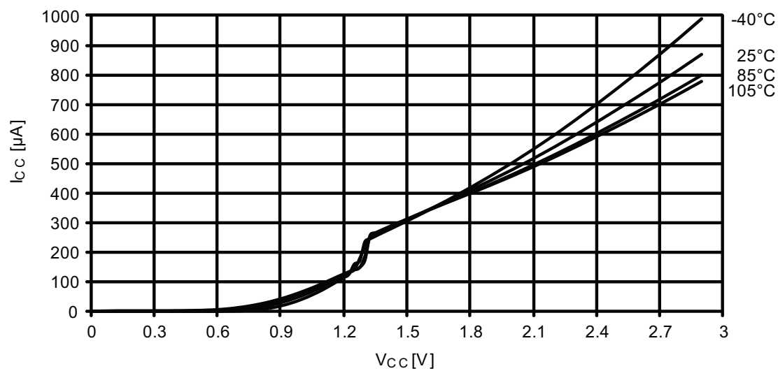
Figure 37-233. Power-on reset current consumption vs. V_{CC} .
