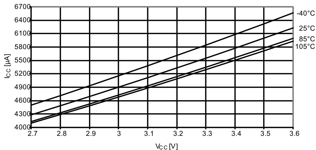
Figure 37-180. Idle mode current vs. V_{CC} .
