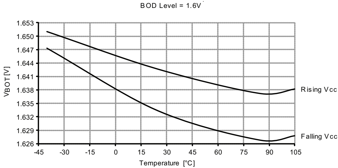
Figure 37-59. BOD thresholds vs. temperature.
