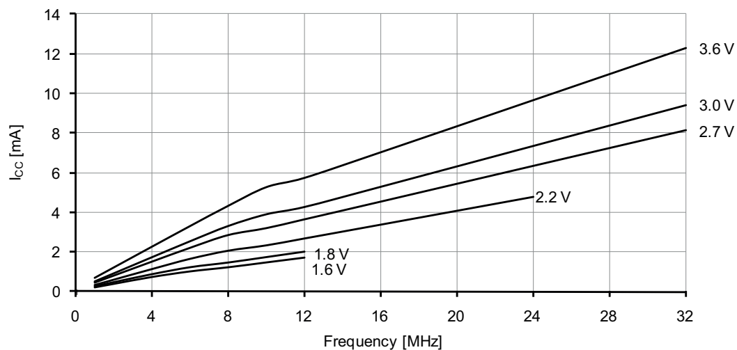
Figure 37-2. Active supply current vs. frequency.
