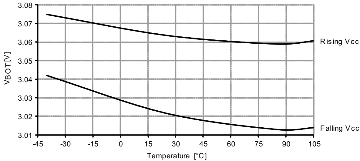
Figure 37-60. BOD thresholds vs. temperature.
