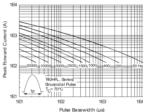
Fig. 37 - Frequency Characteristics
